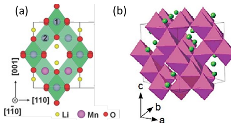
FIGURE 20 – Projection 2D de la structure \text{LiMn}_2\text{O}_4 (a) et structure 3D (b)
